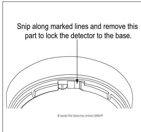
Fig 2. Locking Mechanism
